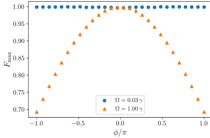
Figure 9. Fidelity achievable with the main text's second quantum-autonomous superconducting-qubit Z gate. In the narrow-bandwidth, strong-coupling regime \Omega \ll \gamma \ll \chi (blue disks), the fidelity is near-perfect. If \Omega is tuned out of this regime (orange triangles), the fidelity worsens as the rotation-angle magnitude |\phi| grows.
